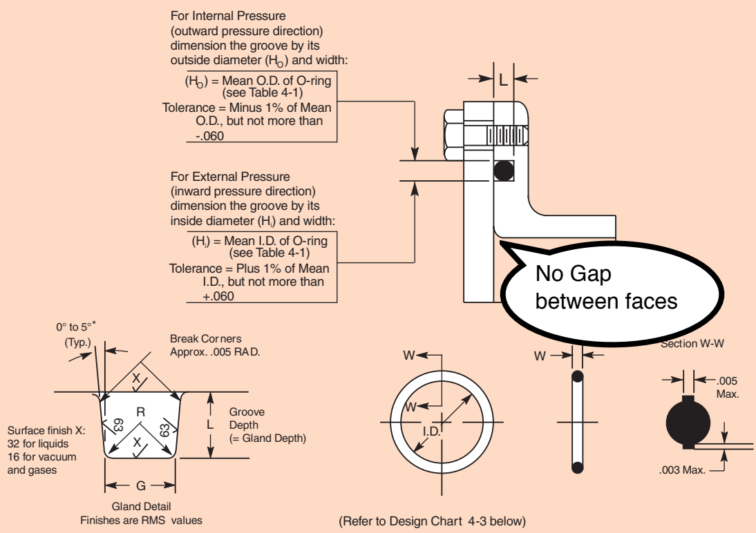
O-Ring Face Seal Glands These dimensions are intended primarily for face type O-ring seals and low temperature applications.
